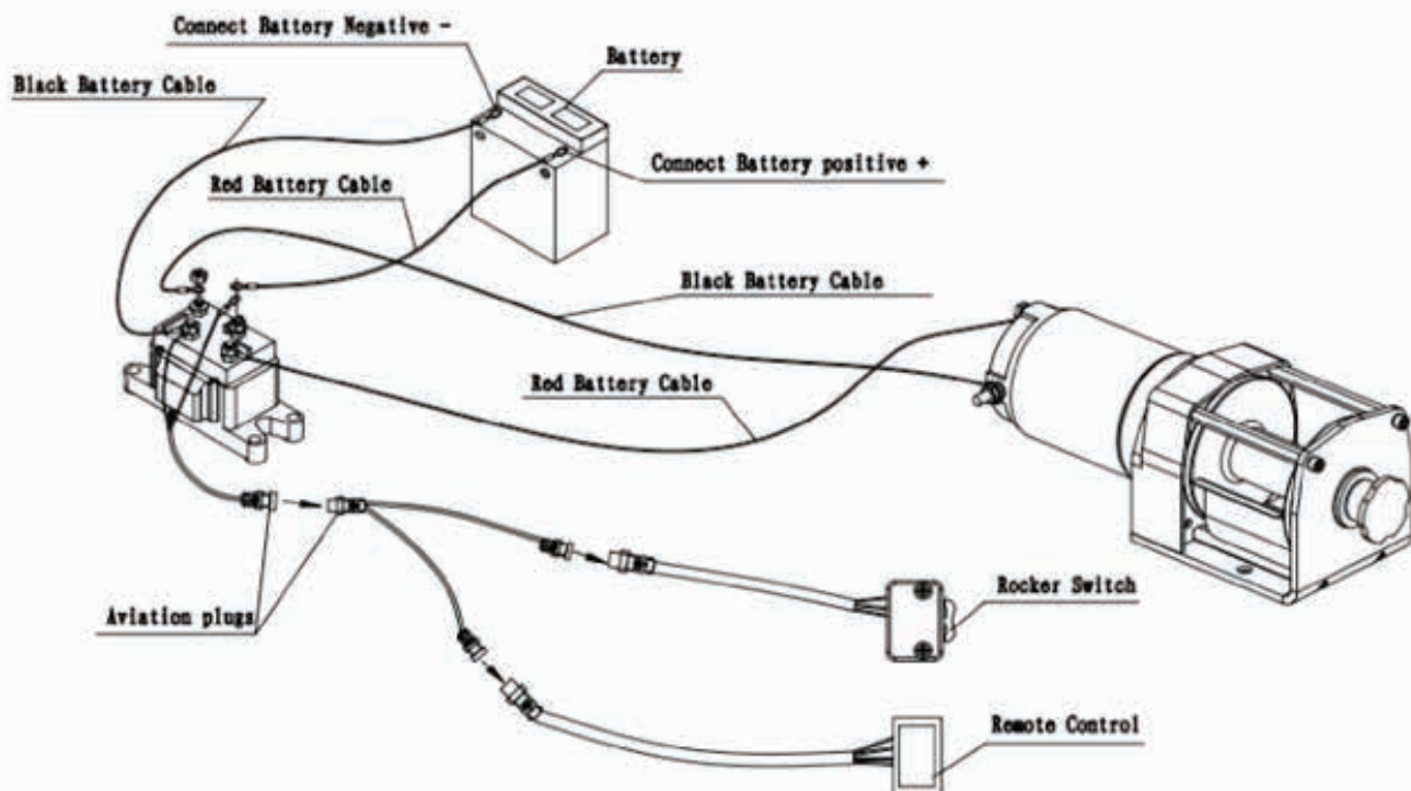
Winch Wiring Diagram
