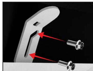
Fig. 9-Lower Bolts
