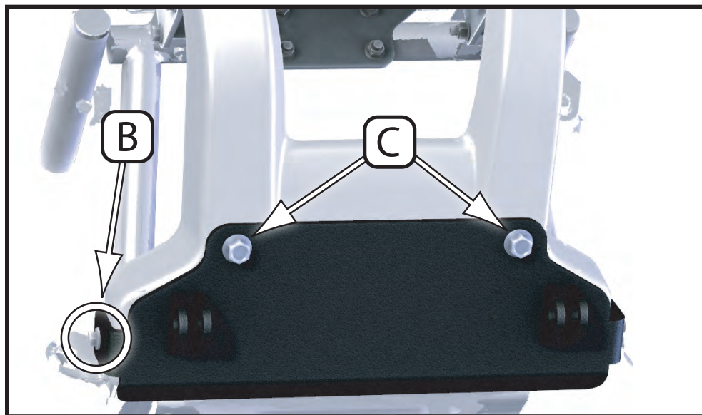
"Figure 3" Mount Plate Install
