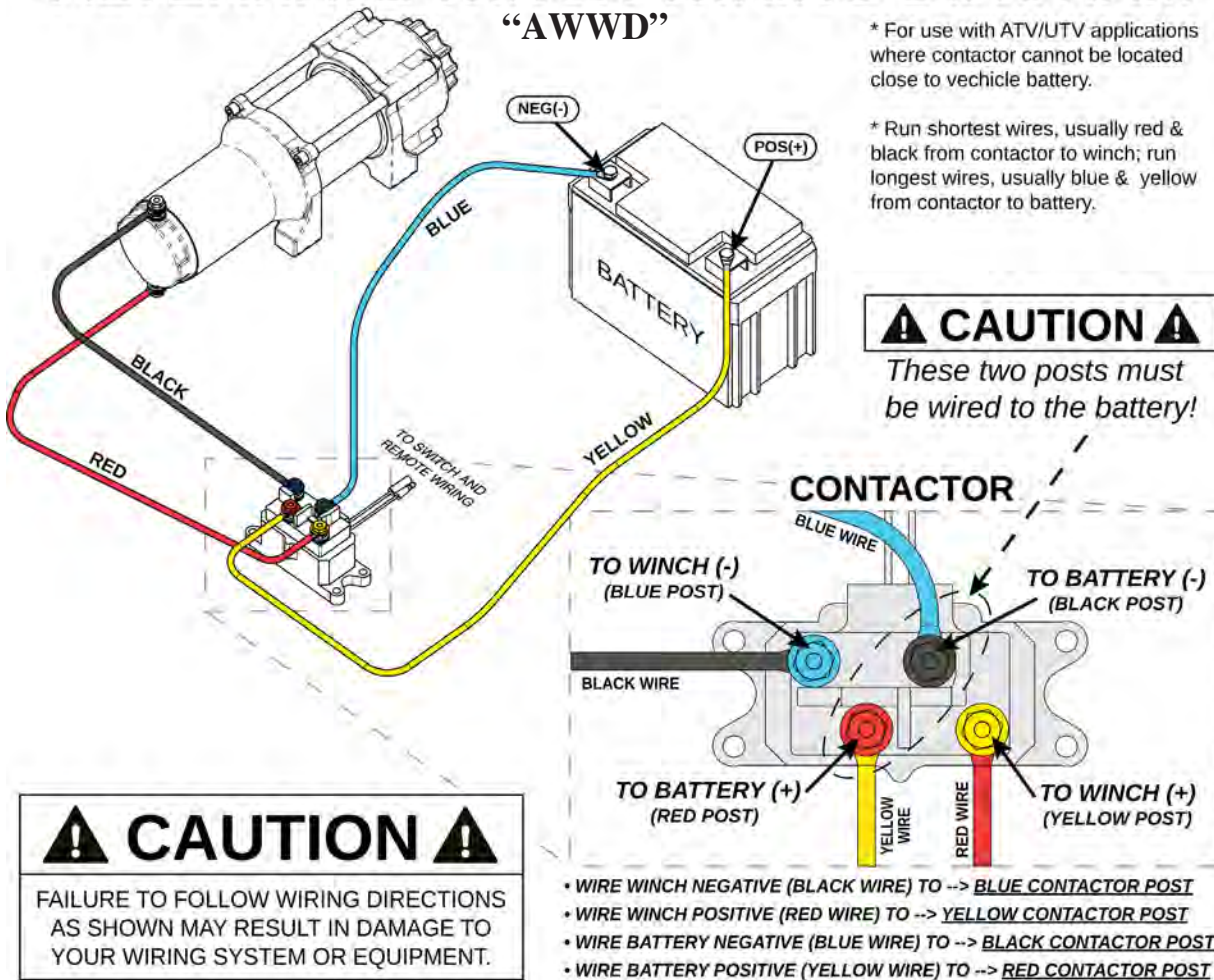
“Figure 12” Alternate Wiring Diagram
