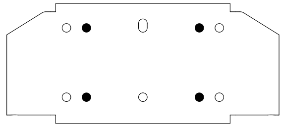
Wide 4 Hole Winch Pattern (6.6" x 3")
