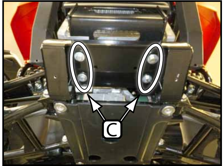
“Figure 5” Winch Mount Bolt Install
