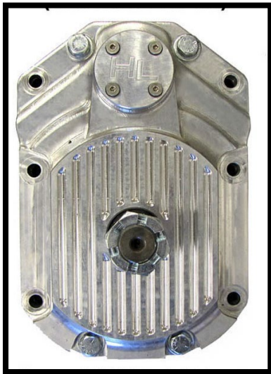
6" Dual Idler 60% Reduction PGL-660DI-GEN1XP-1 Front & Rear Box (4ea) PGLAB-660-DI-P601
