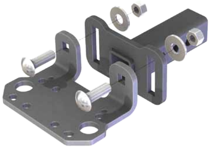
"Figure 1" Bolt Install
