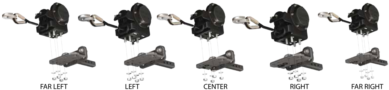
"Figure 2" TigerTail Mounting Positions
