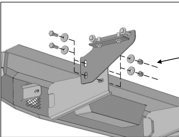
(Fig 10) Attach passenger/right side of Bumper to inside of Frame Bracket
