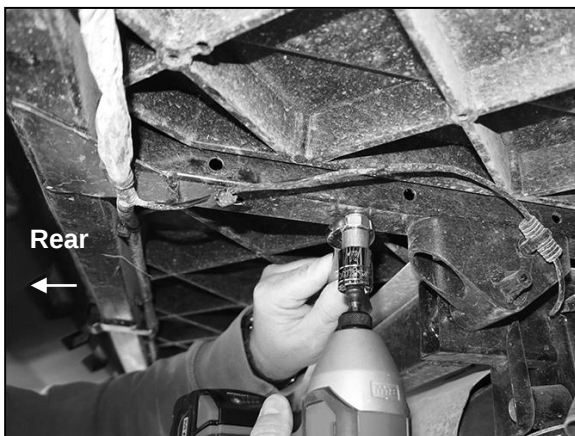
(Fig 5) Insert installation pictured, impact tool use is optional
