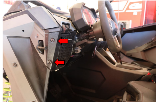
Remove the bolts from the speaker panel.
