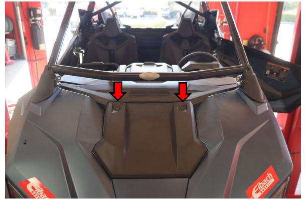
Remove the torx bolts on the upper hood fascia.
