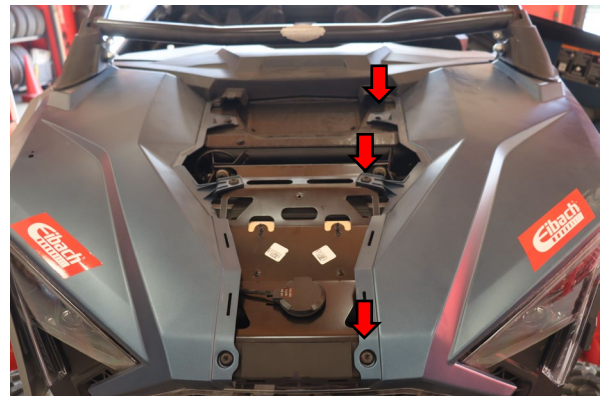
Remove torx bolts and clips securing the side hood fascia.
