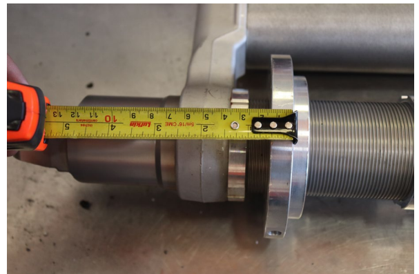
Set the preload collar to 35mm from the bottom of the Resi crossover to the bottom of the preload collar
