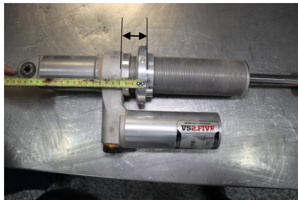
Step 8. Set the preload collar to 40mm measuring from the base of the reservoir housing to the spring flange.
