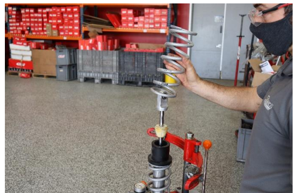
Step 12. Install the Eibach main spring (1000.300.0300S).
