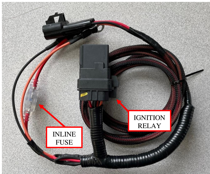
Figure 1: Fuse location.
