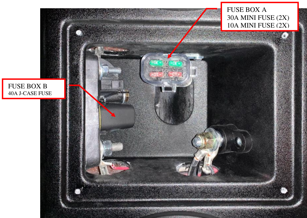
Figure 1: Fuse location.
